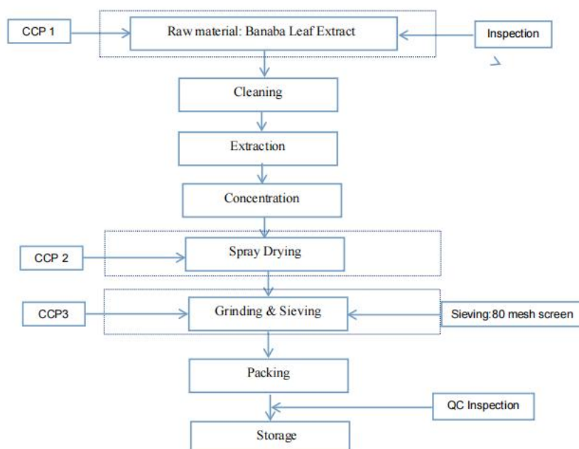
Flow Chart of Banaba Leaf Extract
